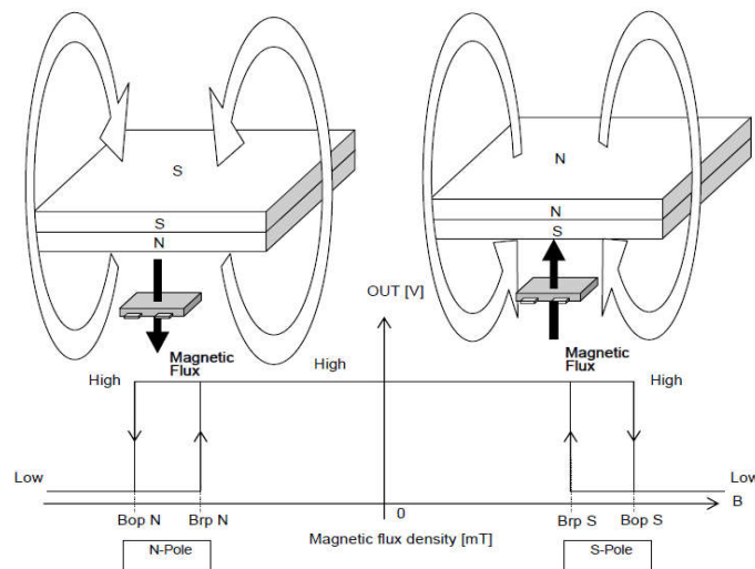
Fig 4, Magnetic Operation Characteristic of AS1803OD
